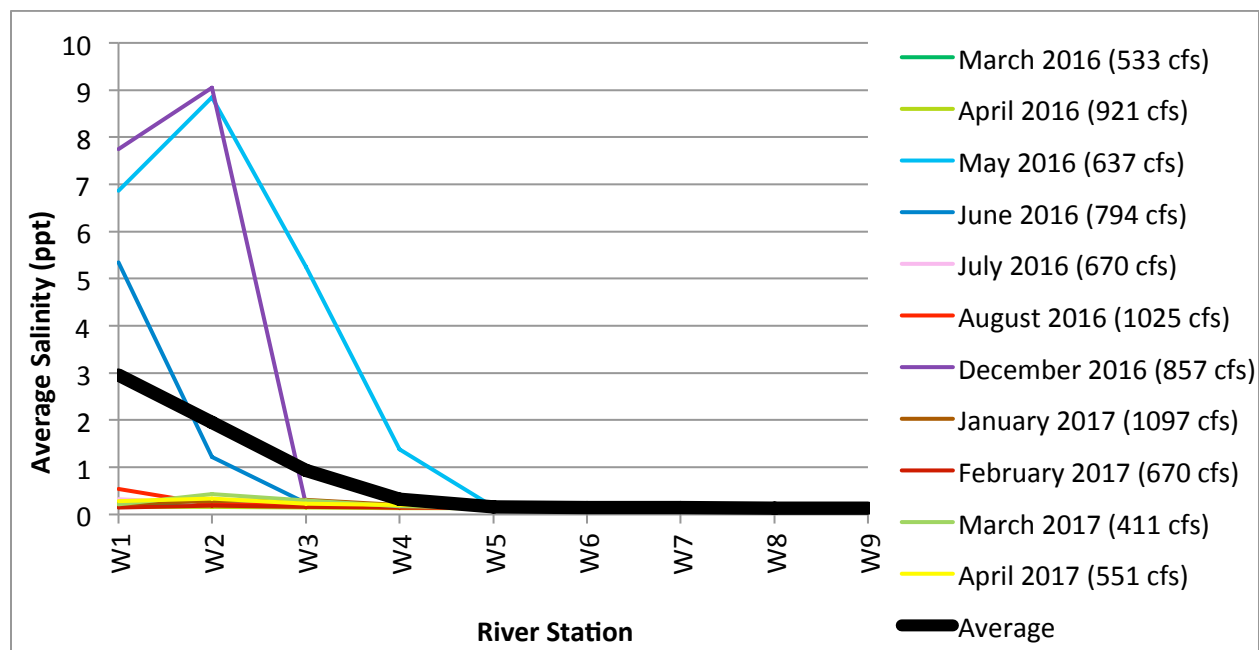
Figure 53: Mean Salinity Observed During In-Situ Water Quality Profile Monitoring Along the Wakulla River. Locations of River Stations are Depicted in Figure 2-3
